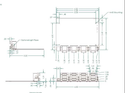
Board Layout for ESU Model
