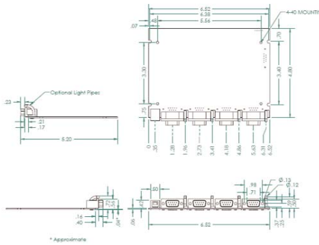
Board Layout for QSU Model
