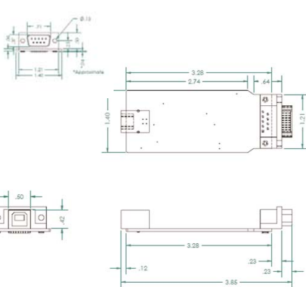
Board Layout for SSU Model
